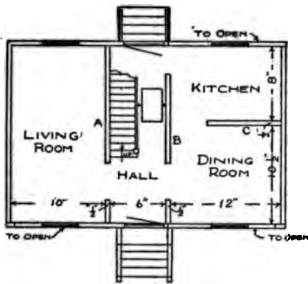
Fig 222 FIRST FLOOR PLAN
